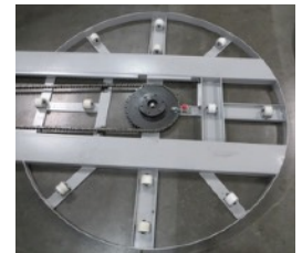
Heavy duty chain drive on turntable with 18 sets of double roller turntable supports.
